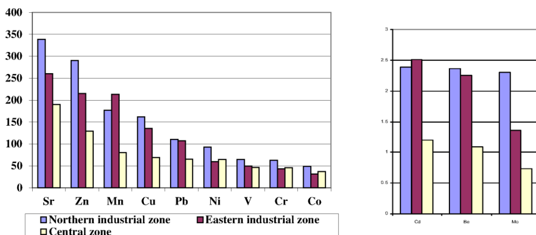
Figure 2. Comparative analysis of the content of the chemical elements in the solid snow fraction of the various zones of Pavlodar
