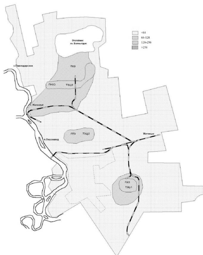
Figure 3. Outline map to arrange the total coefficient ( Z_c ) of pollution in the solid snow cover fraction in Pavlodar
