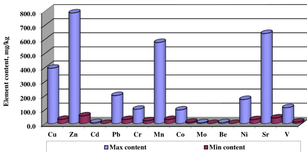
Figure 1. Exceeding of the maximum content of the chemical elements over the minimal one in the solid snow fraction of Pavlodar
